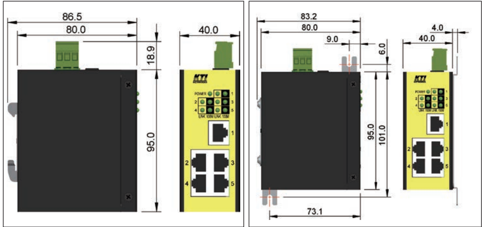
DIN-Rail Dimension
